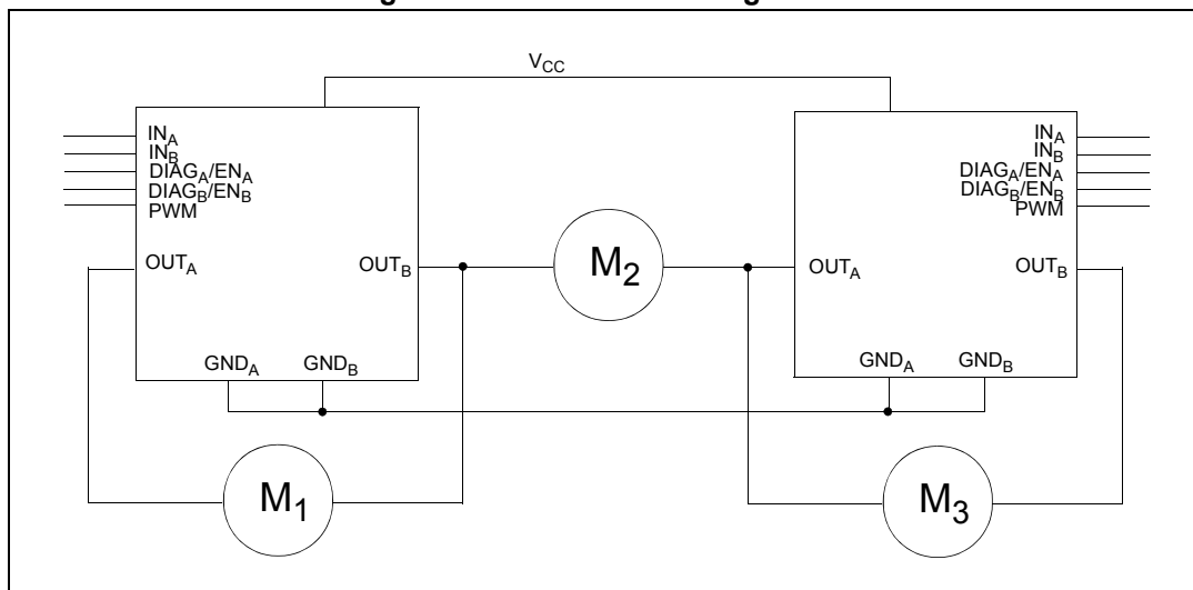
Figure 35. Multi-motor configuration
