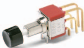
8261SH9AV2BE2 DPDT
