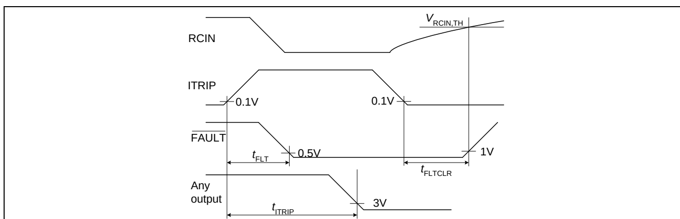
Figure 17 ITRIP-Timing
