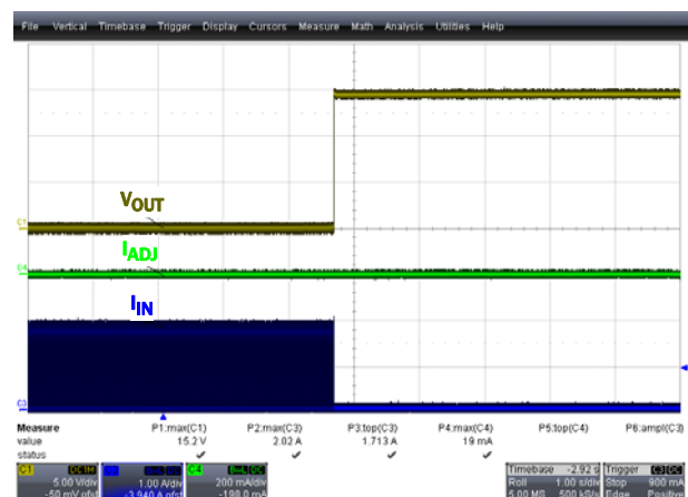
FIGURE 20. SHORT-CIRCUIT RECOVERY
