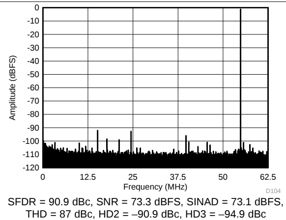
Figure 97. FFT for 70-MHz Input Signal (Dither Off)
