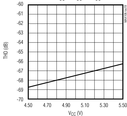
TOTAL HARMONIC DISTORTION vs. V_{CCI} = V_{CCA} = V_{CCD}
