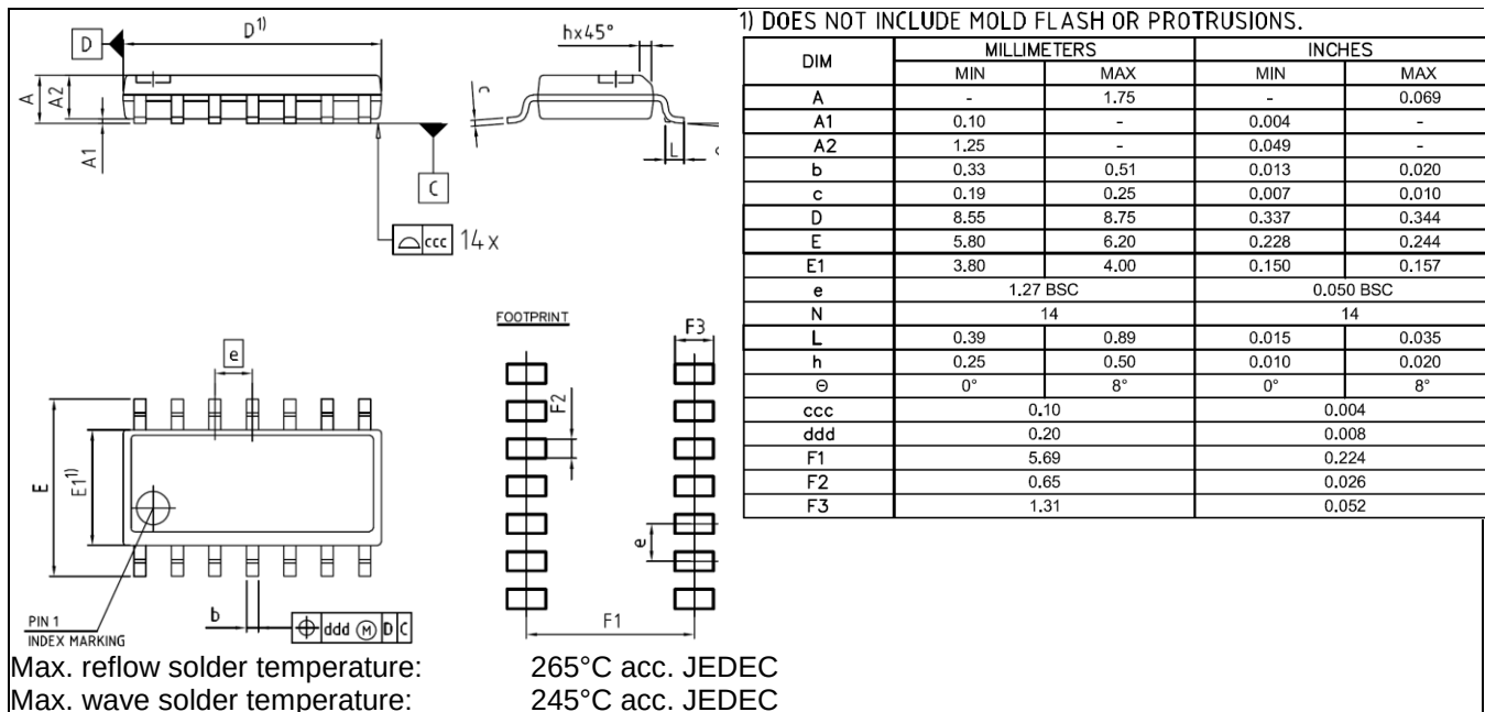
Figure 16 Package drawing
