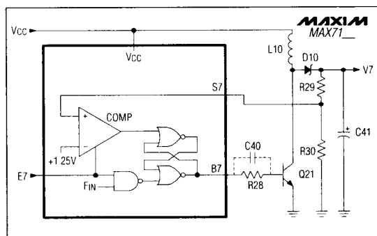
Figure 5. Functional Diagram and Circuit for DC-DC Converter V7
