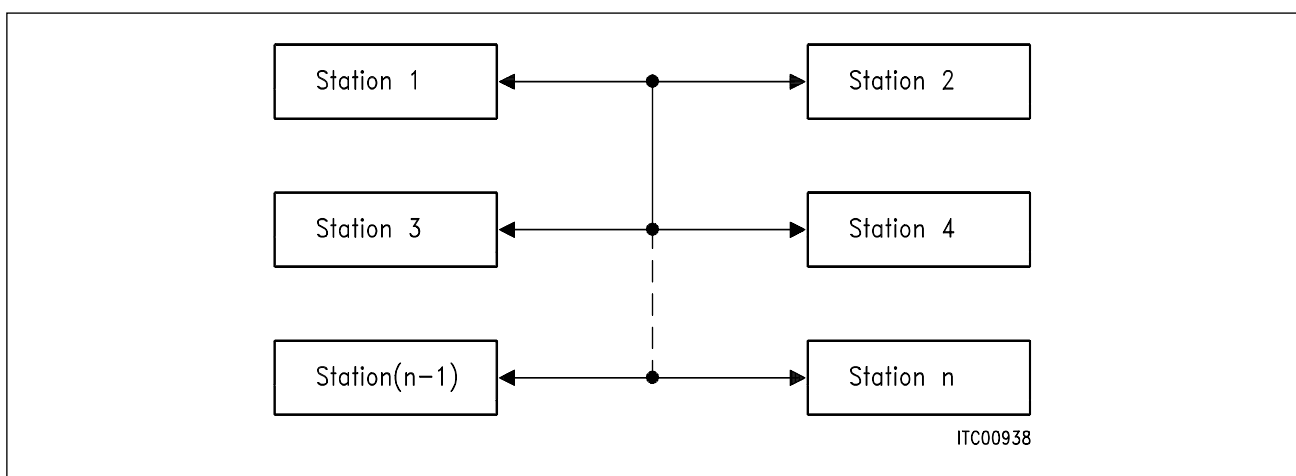
Figure 16c Multimaster Configuration
