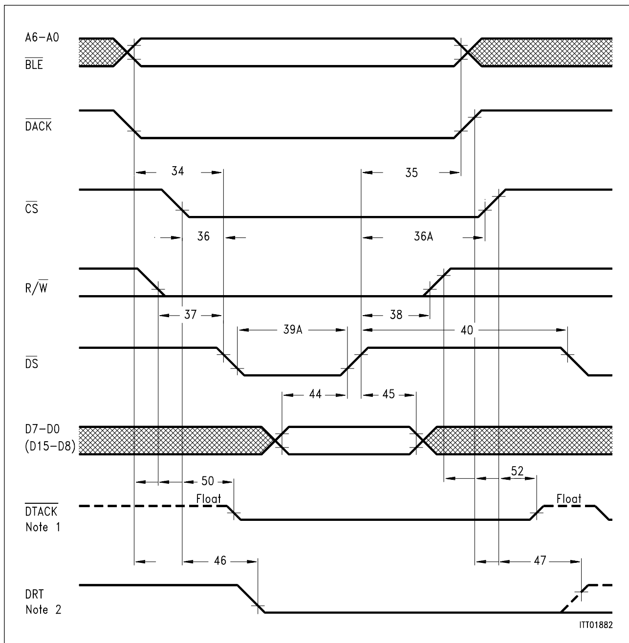
Figure 61 Motorola Write Cycle Timing
