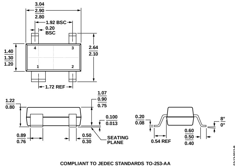
Figure 12. 4-Lead Small Outline Transistor Package [SOT-143] (RA-4)
