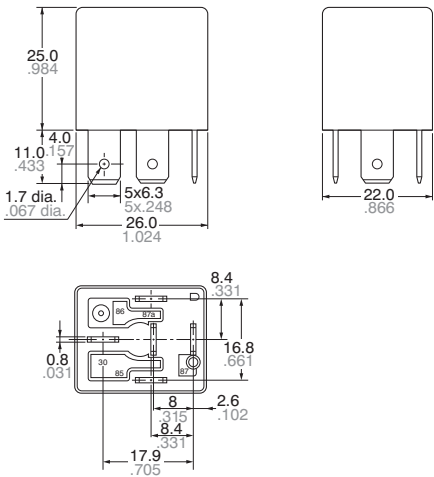
External dimensions
