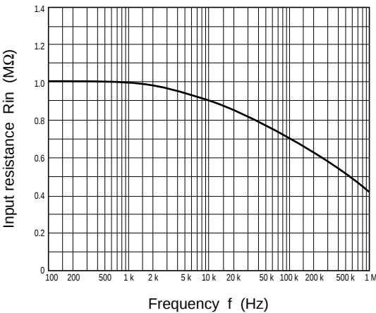
Input Resistance vs. Frequency Characteristics
