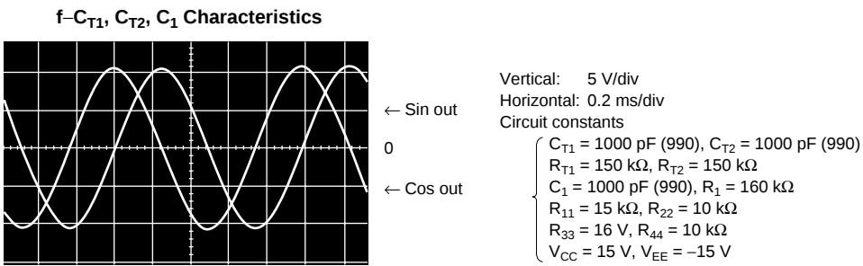
Figure 12 Sine and Cosine Output Waveforms
