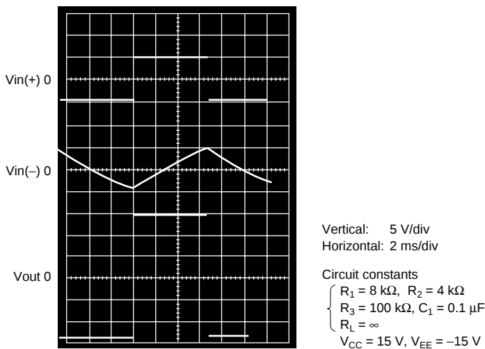
Figure 2 HA17741 Astable Multivibrator Operating Waveform
