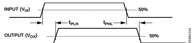
Figure 15. Propagation Delay Parameters
