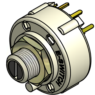
ISOMETRIC
