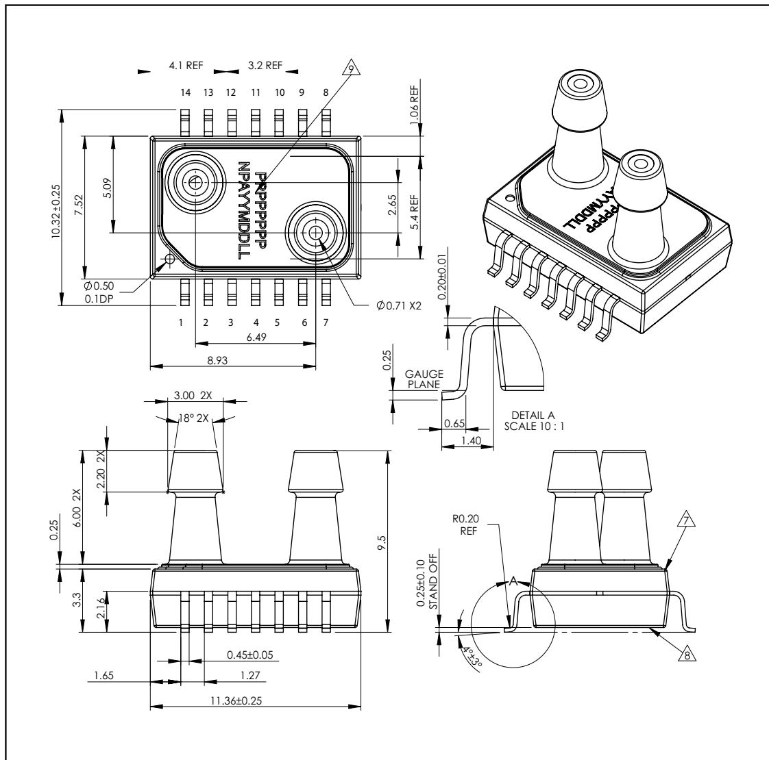
Figure 20: Package Dimensions (mm) - Barbed Fitting, 2 Port (standard version)
