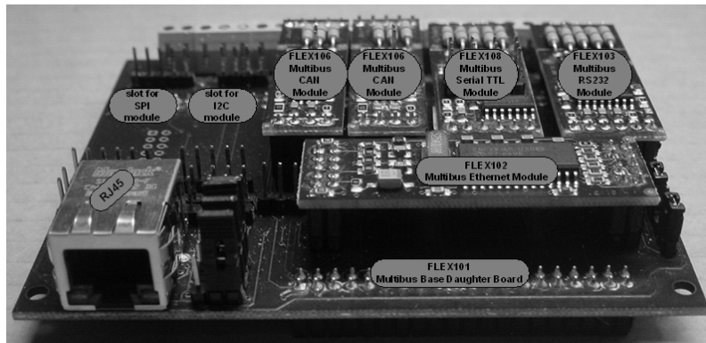
Figure 1: FLEX multibus pack
