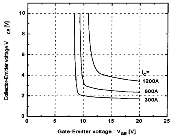
Collector-Emitter vs. Gate-Emitter voltage T_J = 125^\circ\text{C}
