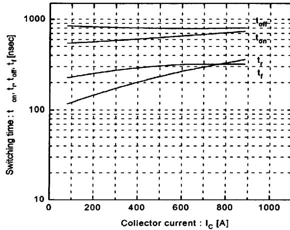
Switching time vs. Collector current V_{CC} = 300\text{V} , R_G = 2.7\Omega , V_{GE} = \pm 15\text{V} , T_J = 125^\circ\text{C}
