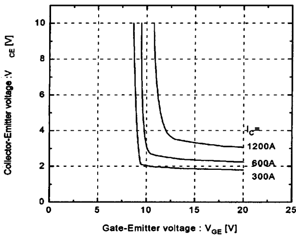
Collector-Emitter vs. Gate-Emitter voltage T_J = 25^\circ\text{C}
