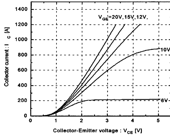
Collector current vs. Collector-Emitter voltage T_J = 125^\circ\text{C}
