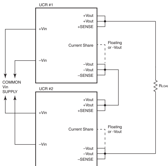
Figure 11. Series Connections
