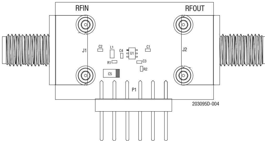
Figure 4. SKY65452-92LF Evaluation Board Assembly Diagram
