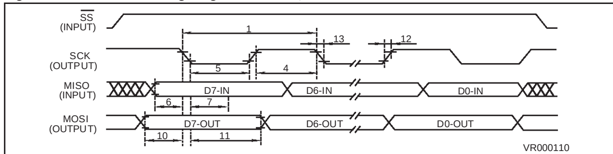
Figure 51. SPI Master Timing Diagram CPHA=0, CPOL=1
