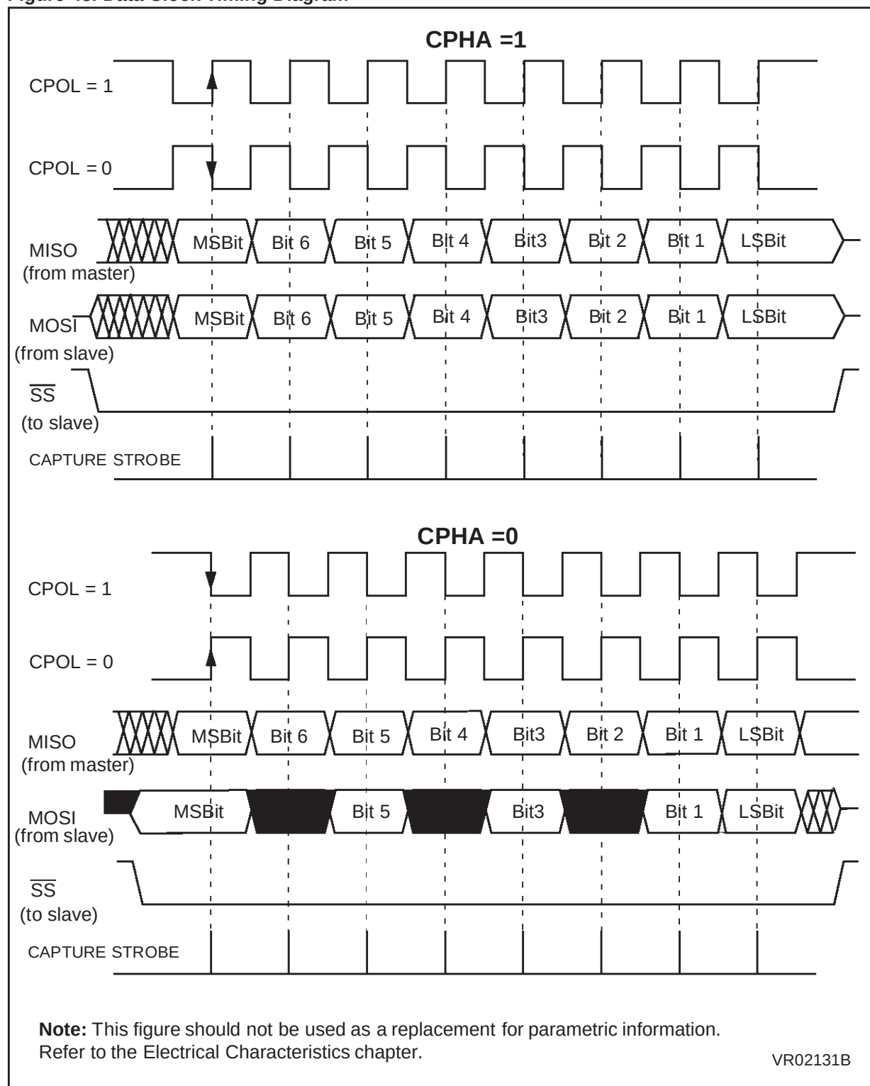
Figure 43. Data Clock Timing Diagram
