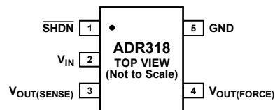
Figure 1. 5-Lead SOT-23
