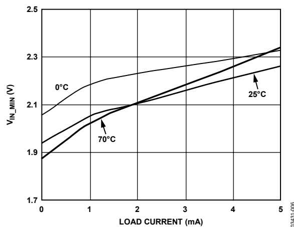
Figure 6. Minimum Input Voltage vs. Load Current
