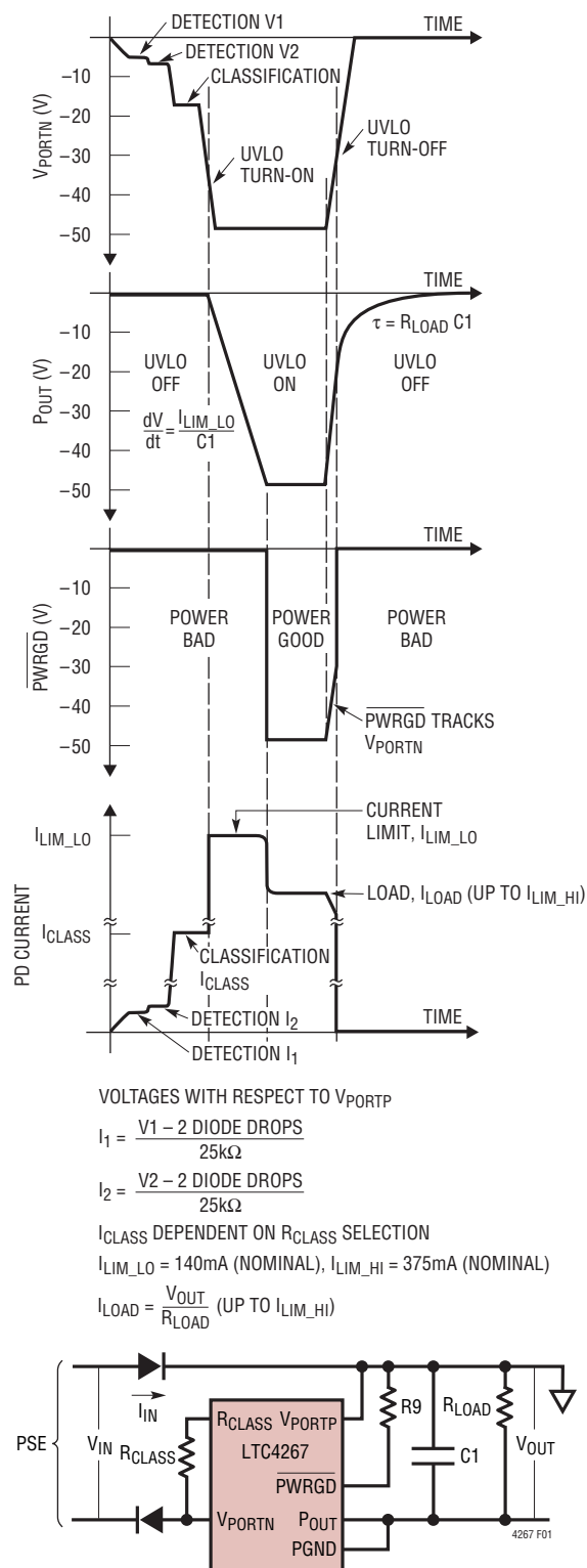
Figure 1. Output Voltage, \overline{\text{PWRGD}} and PD Current as a Function of Input Voltage
