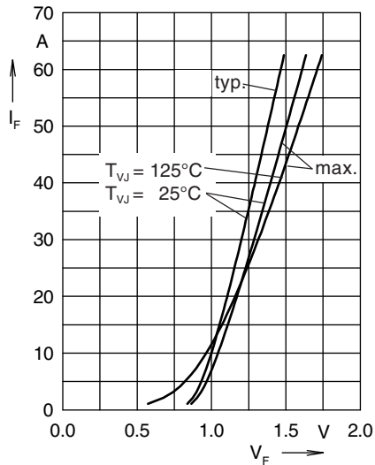
Fig. 3 Forward current vs. voltage drop per diode
