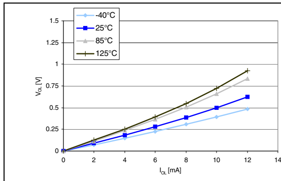
Figure 29. Typ. V_{OL} @ V_{DD} = 3.3 V (high sink ports)
