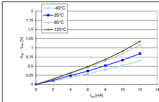
Figure 33. Typ. V_{DD} - V_{OH} @ V_{DD} = 3.3 V (high sink ports)
