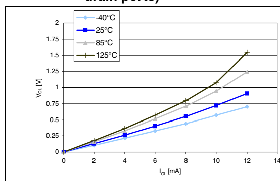
Figure 27. Typ. V_{OL} @ V_{DD} = 3.3 V (true open drain ports)
