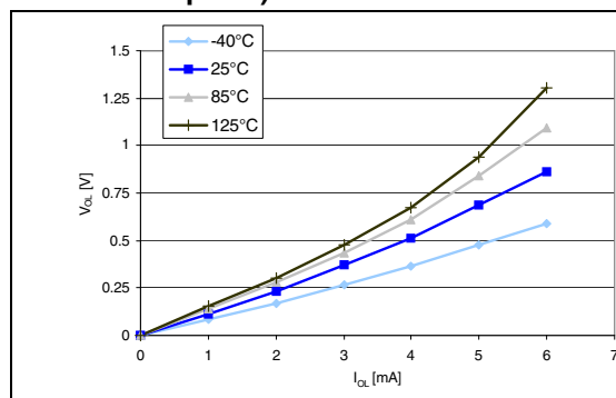
Figure 25. Typ. V_{OL} @ V_{DD} = 3.3 V (standard ports)
