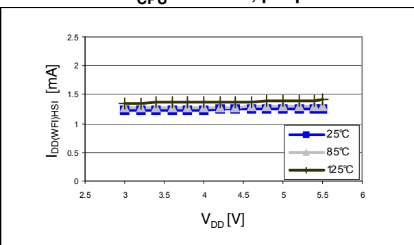
Figure 17. Typ. I_{DD(WFI)HSI} vs. V_{DD} @ f_{CPU} = 16 MHz, peripherals = off
