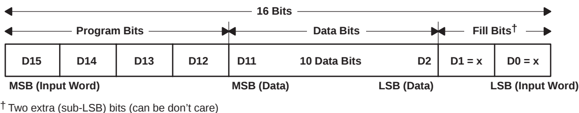
Figure 18. Input Data Word Format
