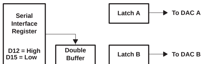
Figure 21. Double-Buffer-Only Write
