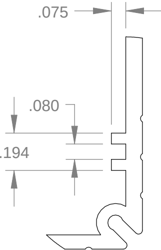
DETAIL C
