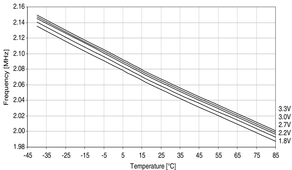
Figure 37-159. 2MHz internal oscillator frequency vs. temperature. DFLL enabled, from the 32.768kHz internal oscillator .
