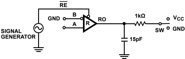
FIGURE 8. RECEIVER PROPAGATION DELAY
