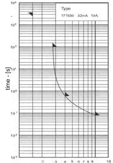
Time-Current Characteristics
