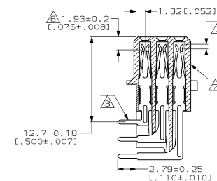
SECTION Y-Y
