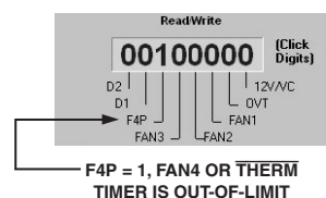
Figure 22. Status Register 2
