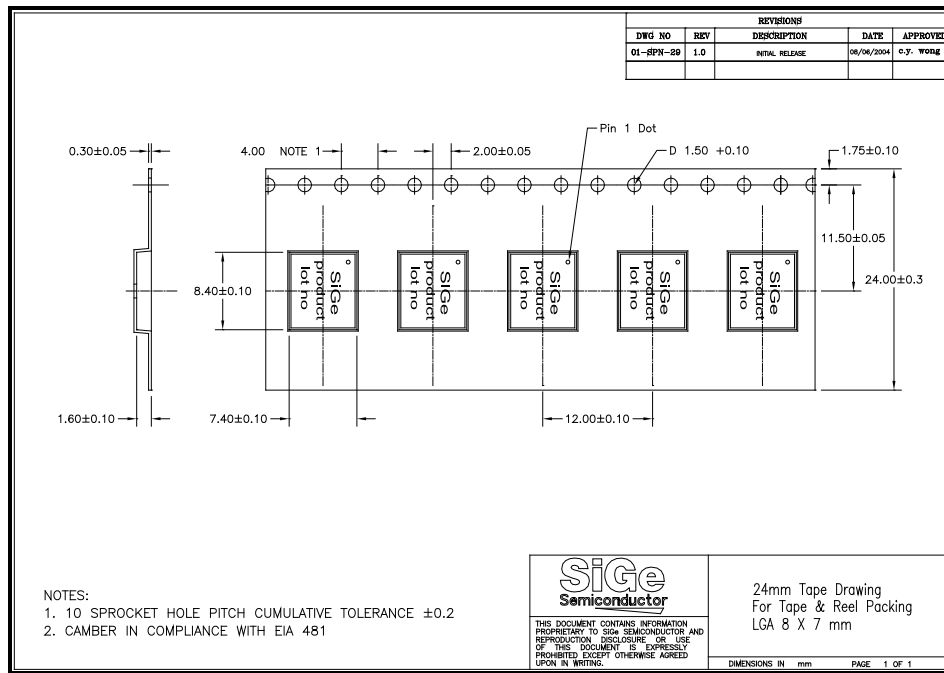
Figure 10: SE2521A80 Tape and Reel Information
