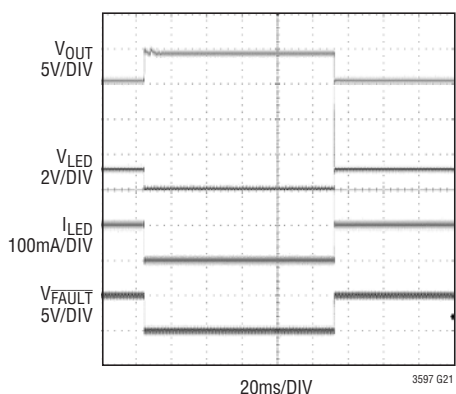
Open LED Fault
