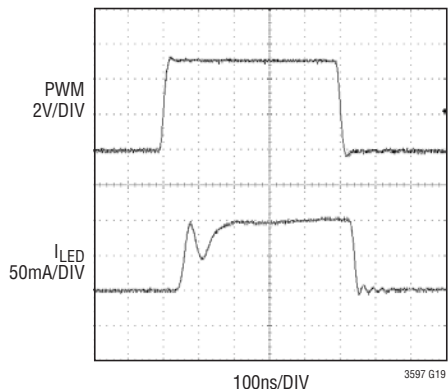
20,000:1 PWM Dimming (100Hz)
