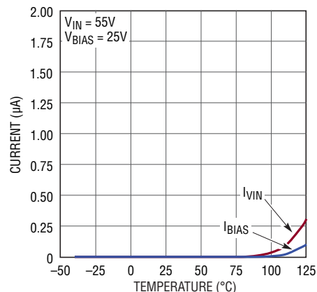
Shutdown Current
