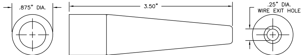
Insulation Boot P/N 9352-color
