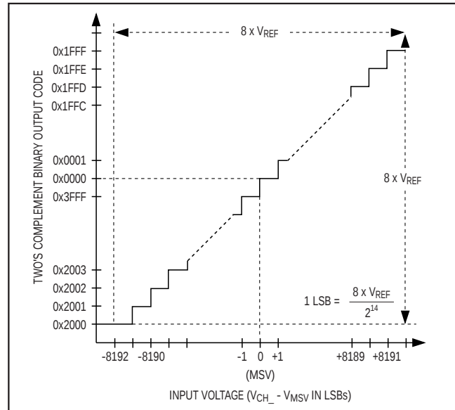
Figure 9. \pm 10\text{V} Bipolar Transfer Function
