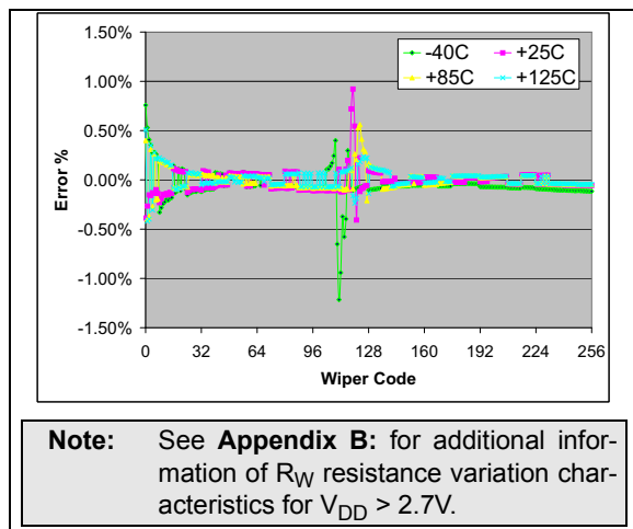
FIGURE 2-38: 10 kΩ – Worst Case R_{BW} from Average R_{BW} ( R_{BW0} - R_{BW3} ) Error (%) vs. Wiper Setting and Temperature ( V_{DD} = 1.8\text{V} , I_W = 150\text{ }\mu\text{A} ).
