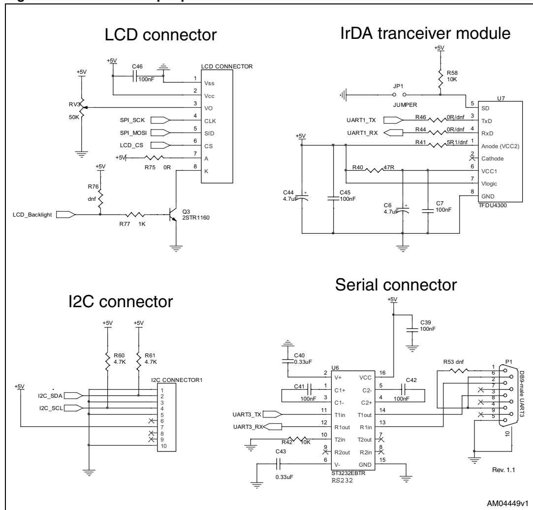
Figure 18. Schematic - peripherals
