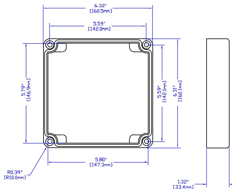
VIEW OF LID (INSIDE)
