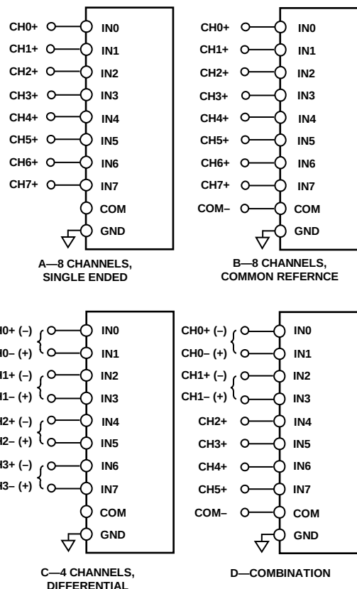
Figure 29. Multiplexed Analog Input Configurations
