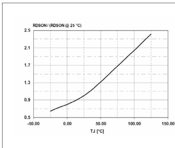
Figure 14. Power MOSFET on-resistance vs T_J Figure 15. Power MOSFET break down voltage vs T_J
