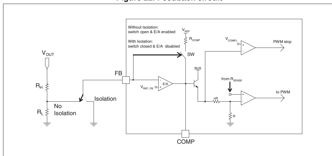
Figure 22. Feedback circuit
