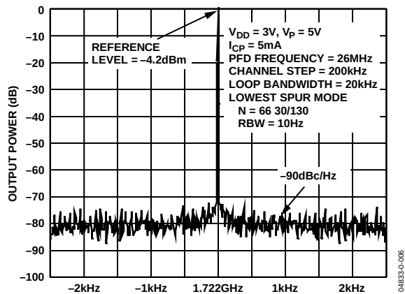
Figure 7. Phase Noise (Lowest Spur Mode)
