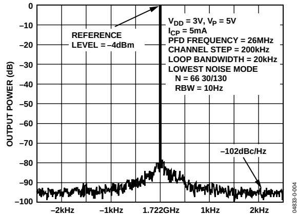
Figure 5. Phase Noise (Lowest Noise Mode)
