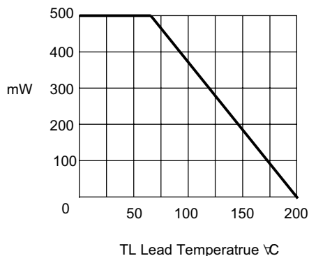
Figure 2 - Derating Curve
