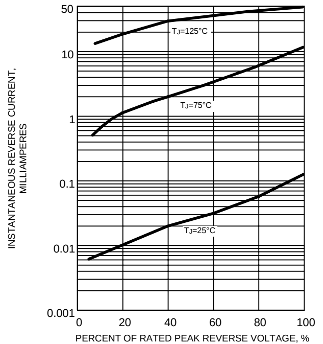
FIG. 4 - TYPICAL REVERSE CHARACTERISTICS PER LEG
