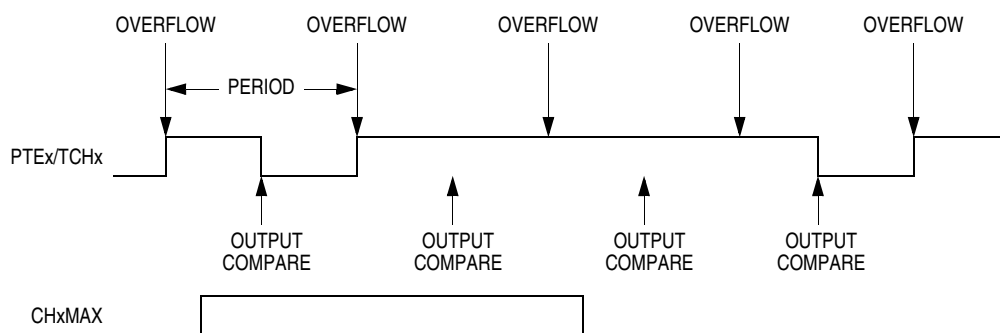
Figure 17-8. CH x MAX Latency
