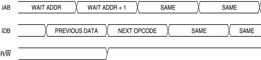
Figure 15-12. Wait Mode Entry Timing
