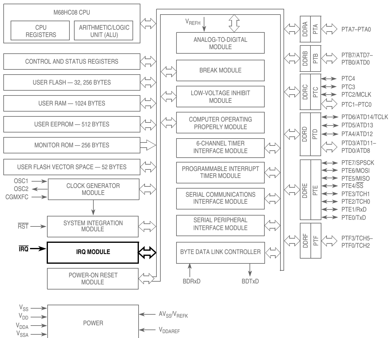
Figure 10-1. Block Diagram Highlighting IRQ Block and Pins
