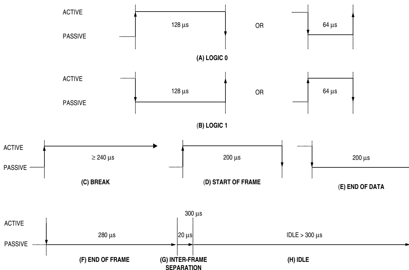
Figure 4-7. J1850 VPW Symbols with Nominal Symbol Times
