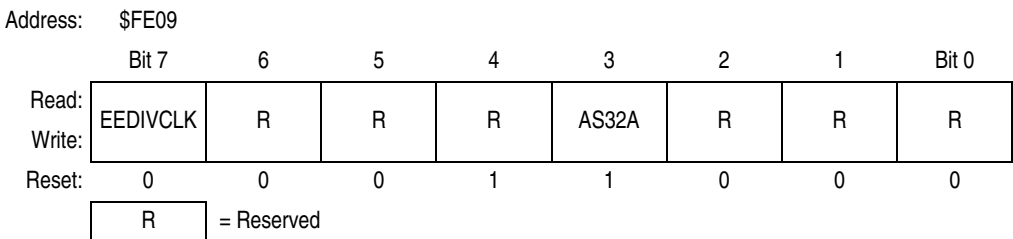
Figure 7-1. Configuration Register (CONFIG2)
