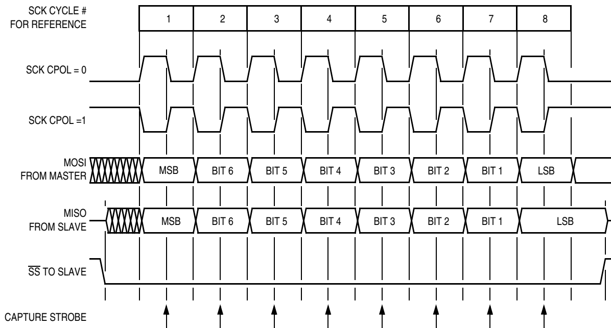
Figure 16-5. Transmission Format (CPHA = 1)
