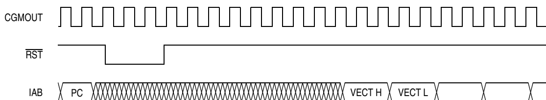
Figure 15-4. External Reset Timing
