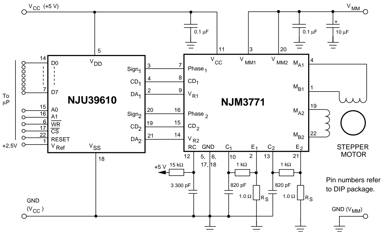
Figure 14. Typical application in a microprocessor based system.
