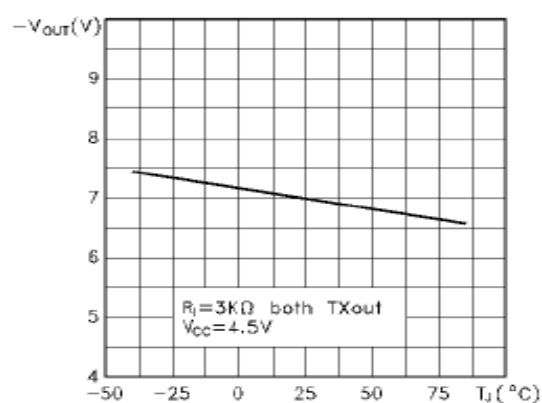
Figure 8: Low level output voltage swing vs temperature
