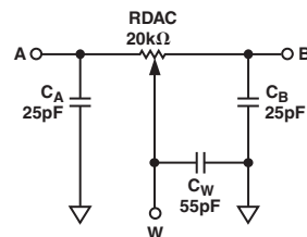
Figure 26. RDAC Circuit Simulation Model for RDAC = 20 k \Omega
