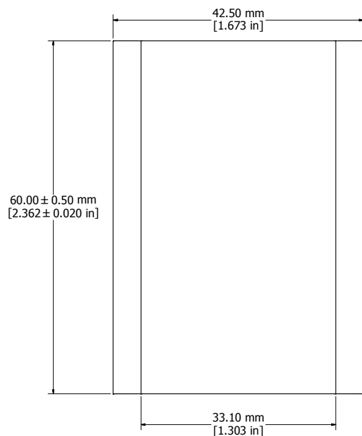
EXTRUSION PROFILE
