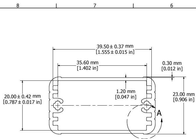
EXTRUSION PROFILE
