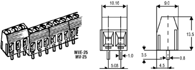
MVE-25. 5 mm (0.197") pin spacing, 15 A, 300 V, 30-14 AWG. 13.5 mm (0.53") high. 0.8 × 1.0 mm (0.032 × 0.039") rectangular pins. Color: Green.
