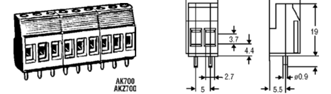
AK700. 5 mm (0.197") pin spacing, 15 A, 300 V, 22-12 AWG. 19 mm (0.75") high. 0.9 × 0.9 mm (0.035 × 0.035") square pins. Color: Green.
