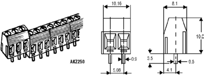
AKZ250. 5.08 mm (0.200") pin spacing, 10 A, 300 V, 26-14 AWG†. 10 mm (0.39") high. 0.5 × 0.9 mm (0.019 × 0.035") rectangular pins. Color: Green.
