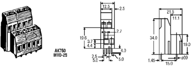
AK750. 5 mm (0.197") pin spacing, 15 A, 300 V, 22-12 AWG. Double level, 2nd level offset 2.5 mm (0.10") left, 34 mm (1.34") high. 0.9 × 0.9 (0.035 × 0.035") square pins. Color: Green.
