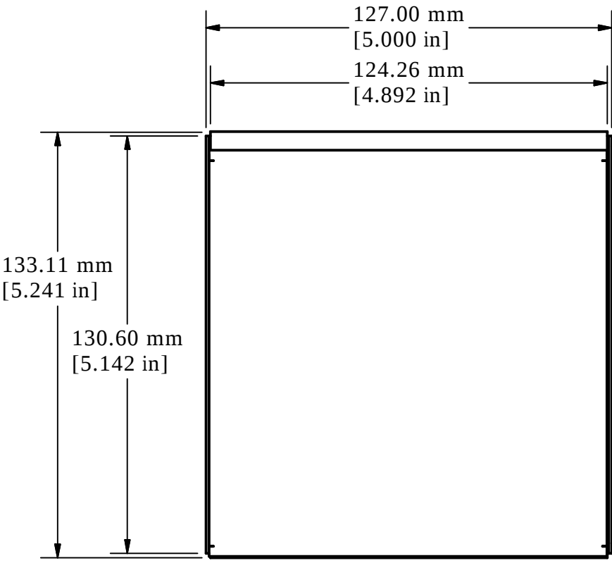
BOTTOM VIEW OF ASSEMBLY
